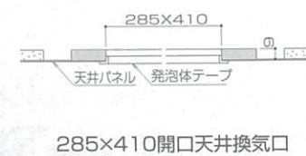
285×410開口天井換気口
